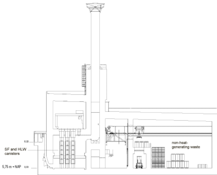
Figure 1 Cross-section of the HABOG facility
