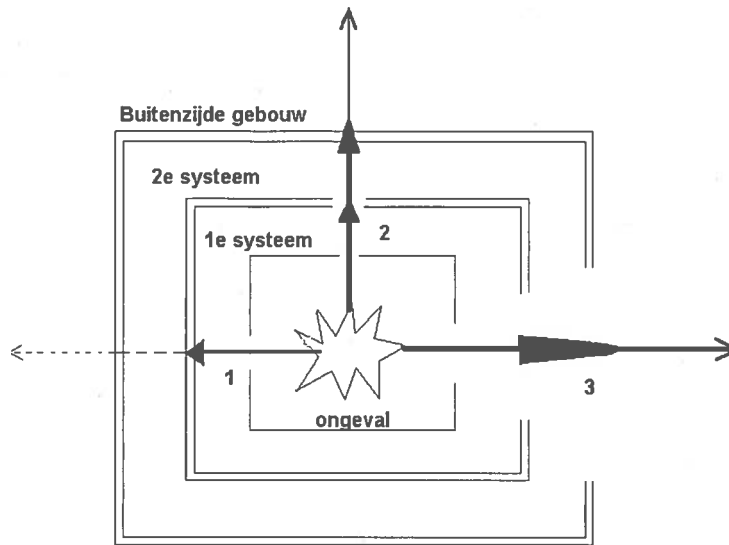
figuur 2 Filosofie "defence in depth" ongevalsituaties
